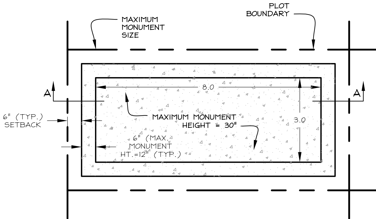
PLAN VIEW
