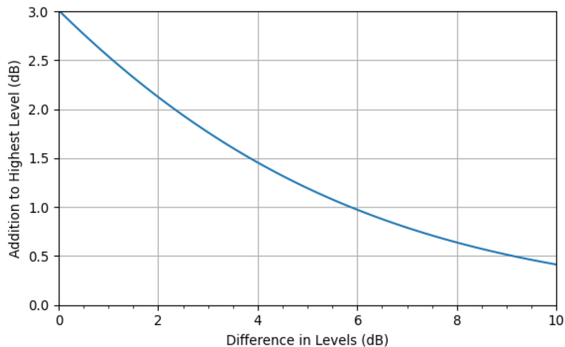
Figure 5.3. Decibel Addition
