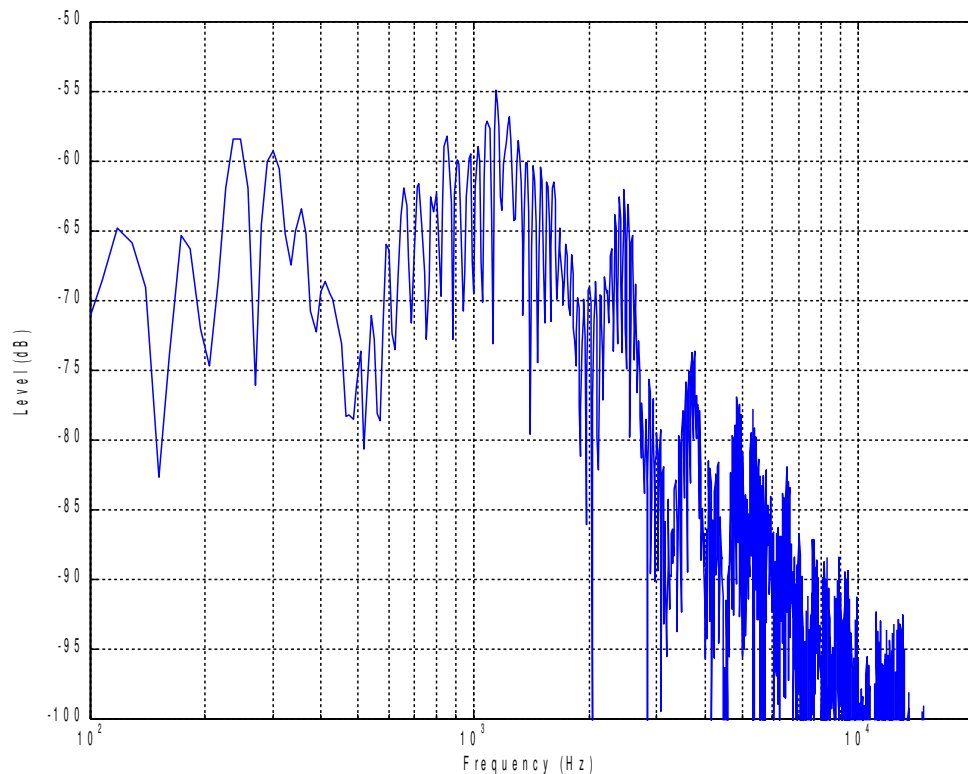
Figure 6.3. Spectral Response of a Dull Hit
