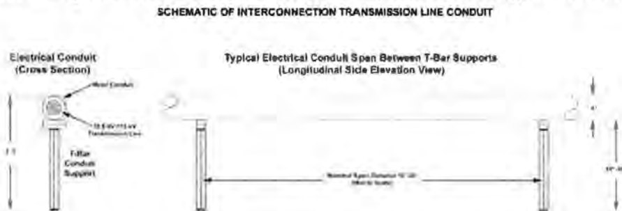
Figure 11: Schematic of Interconnection Transmission Line Conduit
